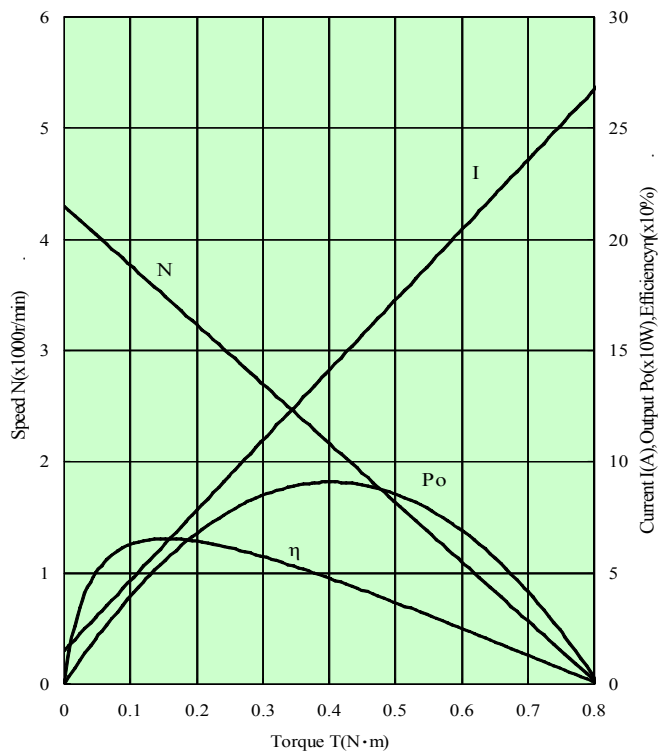
Performance:YA-362(DC12V)
